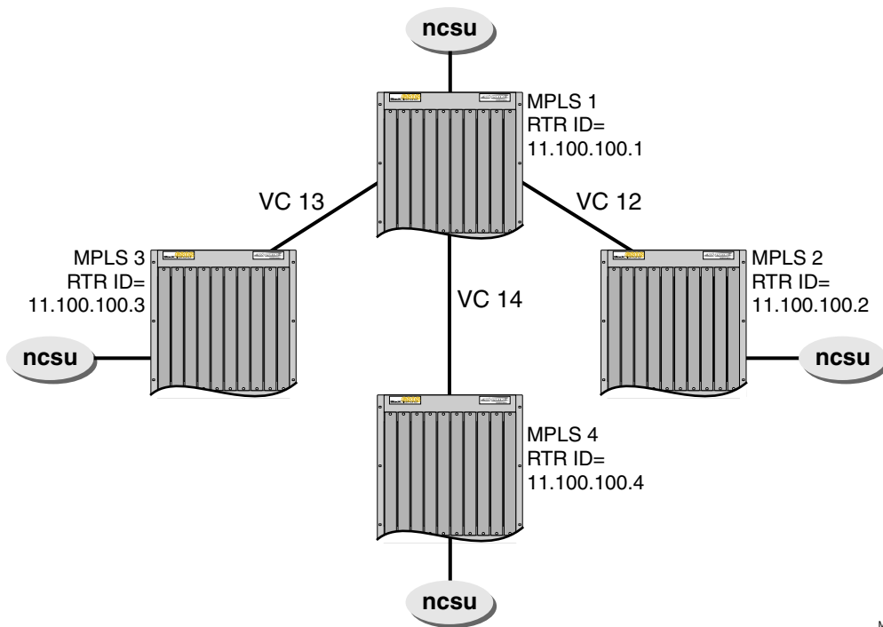
Figure 7-3: Hub and spoke configuration example
