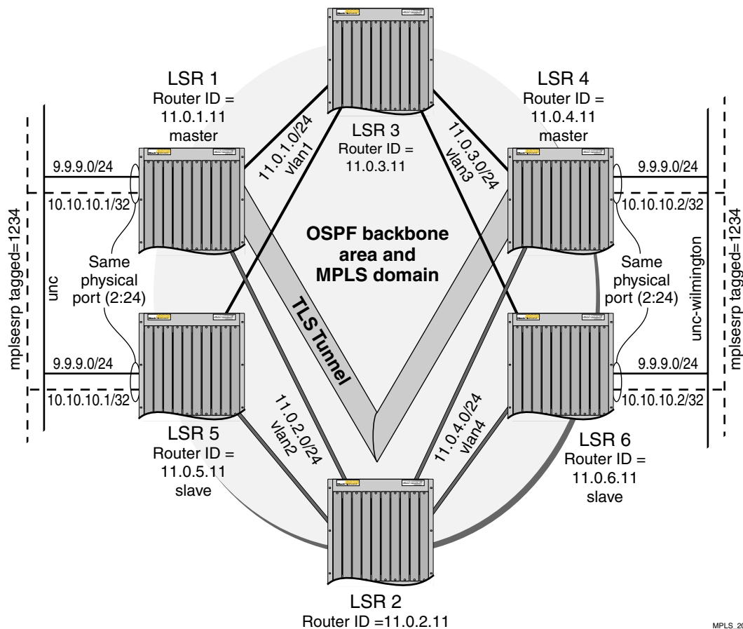
Figure 7-7: TLS configuration example using ESRP
