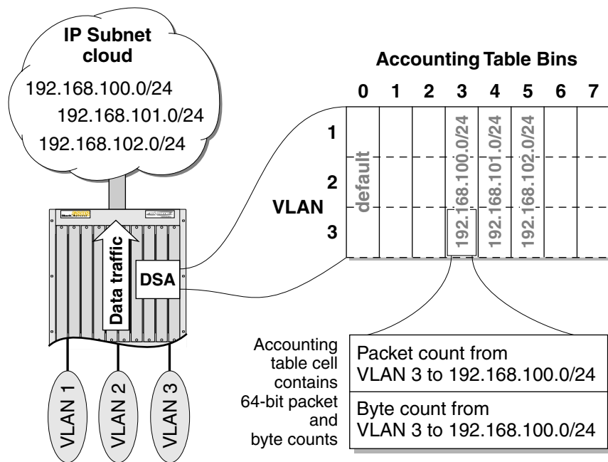
Figure 8-1: Destination-sensitive accounting based on destination IP subnets
