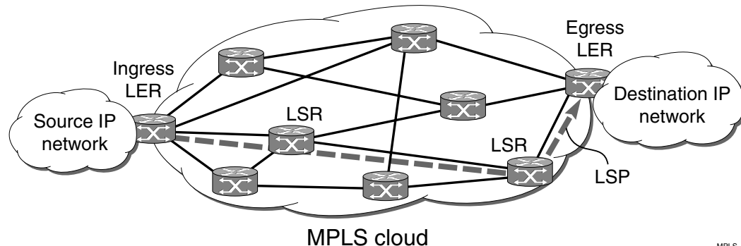
Figure 3-1: MPLS network
