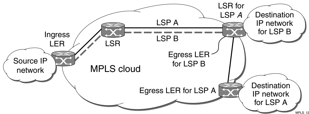
Figure 3-2: LSR types
