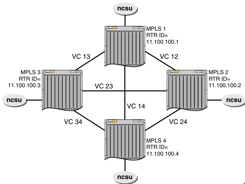
Figure 7-2: Full mesh configuration example
