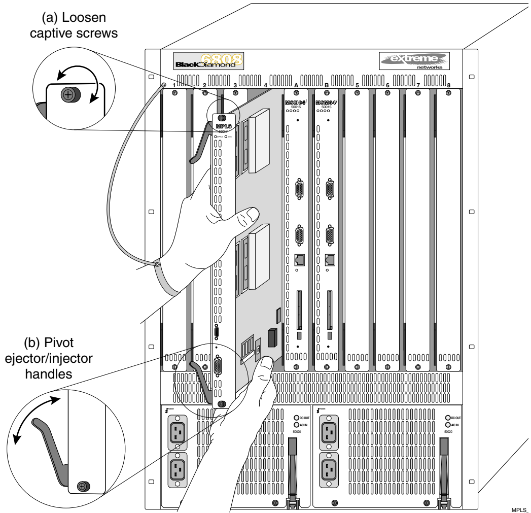
Figure 2-2: Inserting and securing an MPLS module
