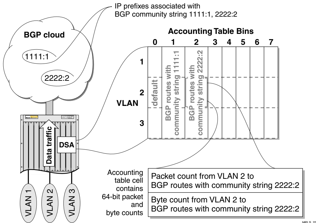
Figure 8-2: Destination-sensitive accounting based on BGP community strings
