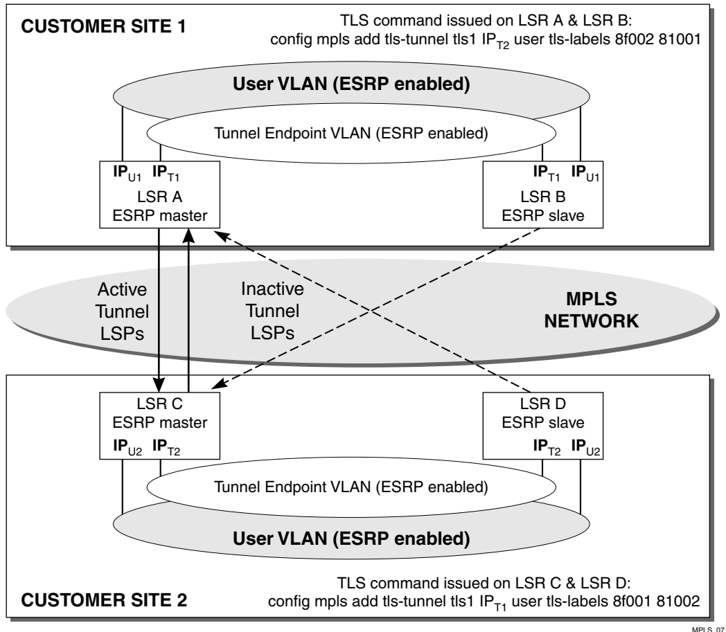
Figure 7-6: Tunnel endpoint VLANs
