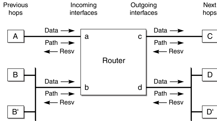
Figure 5-1: RSVP Messages
