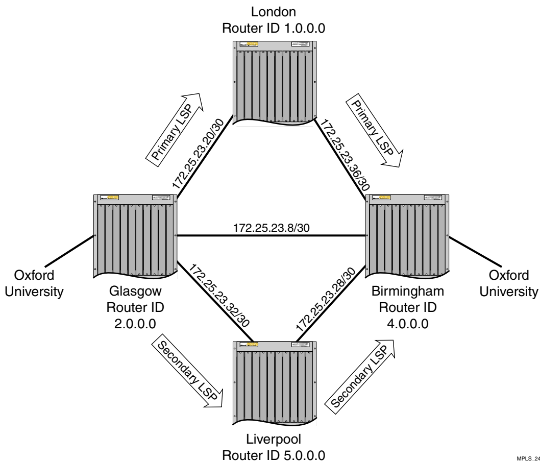
Figure 5-2: RSVP-TE Configuration Example
