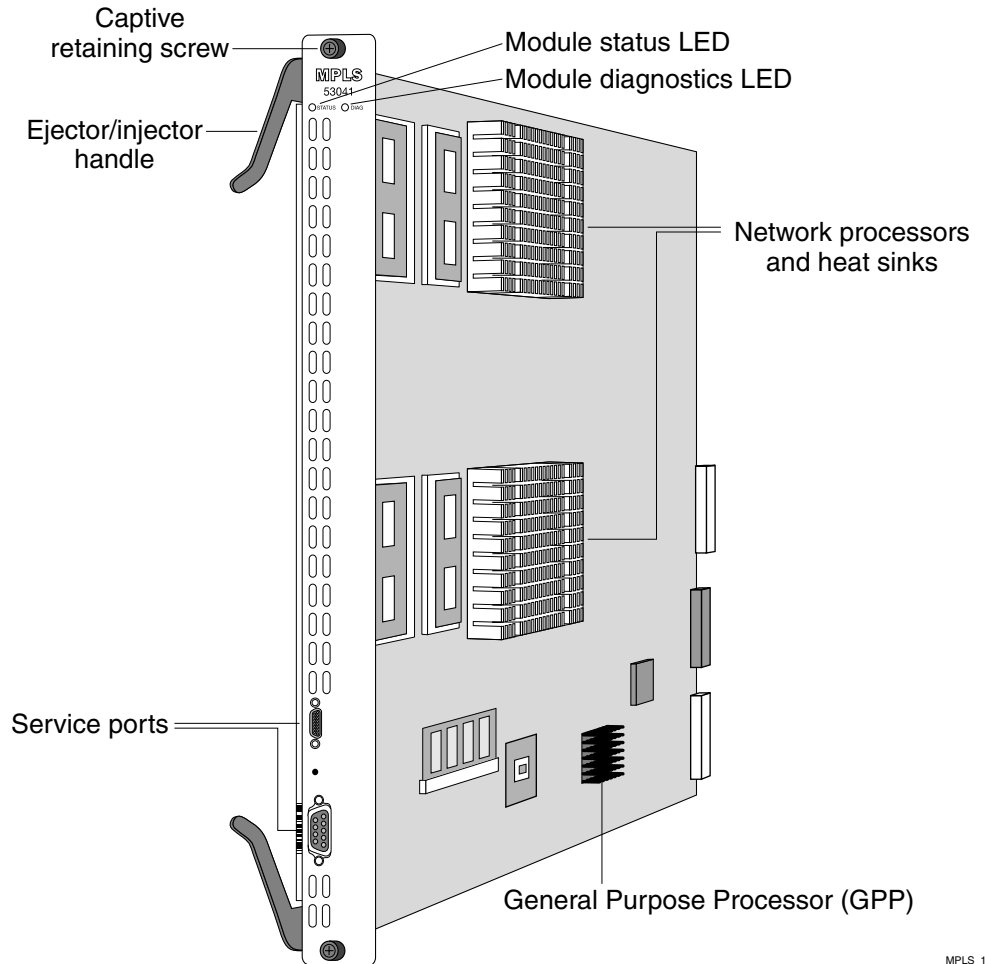
Figure 1-1: MPLS module
