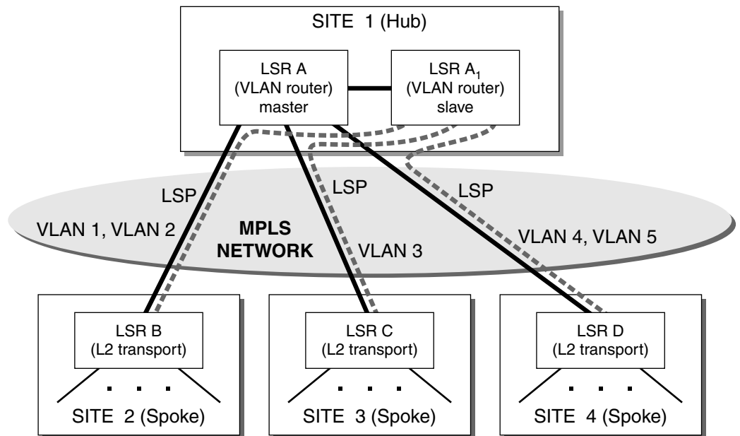
Figure 7-5: Using ESRP with TLS
