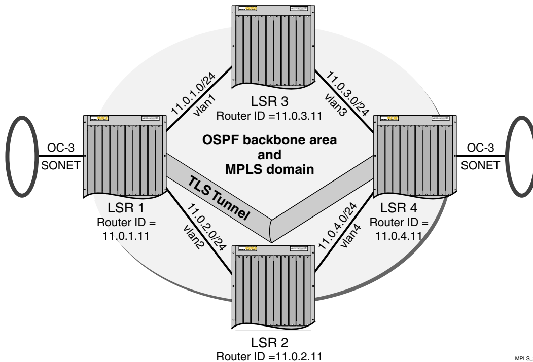
Figure 7-4: TLS configuration example using PPP transparent mode
