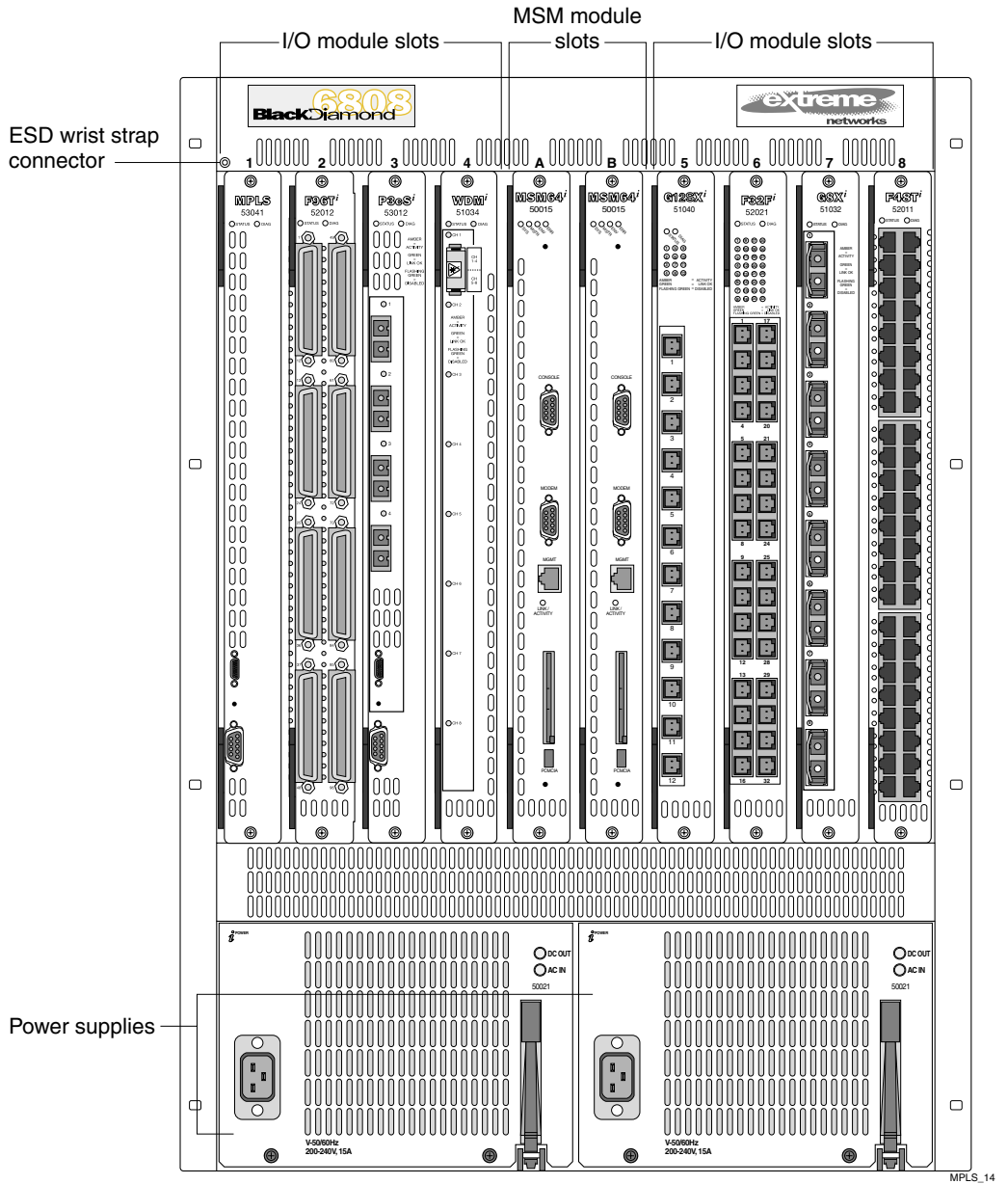
Figure 2-1: Slot locations in a BlackDiamond 6808 series chassis
