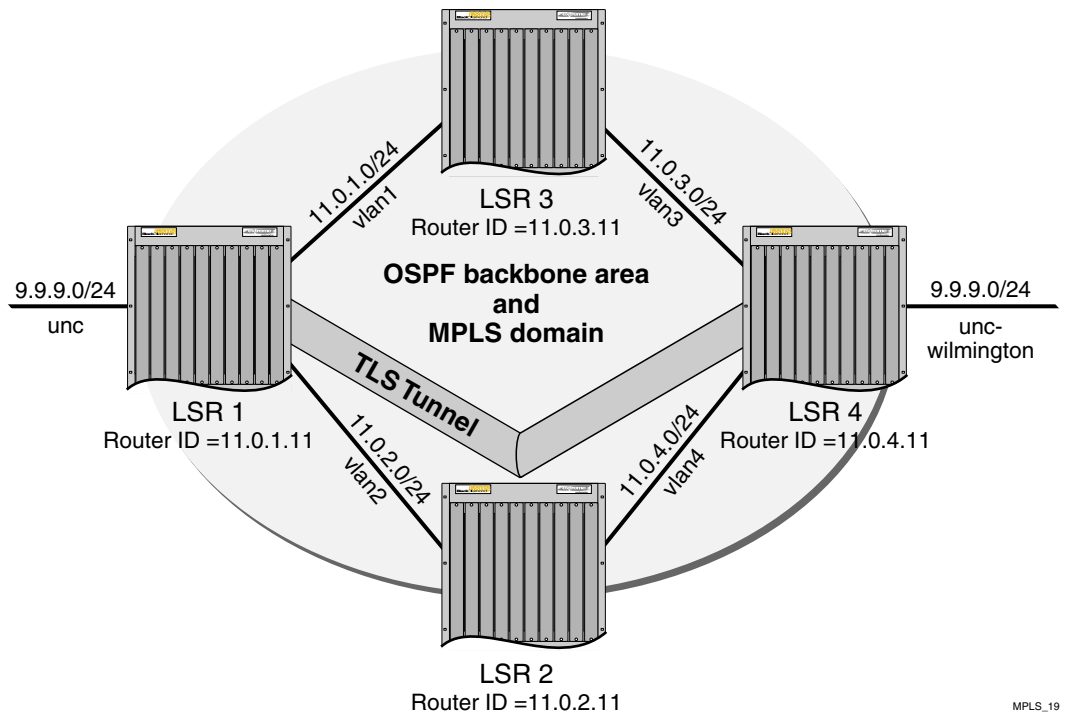
Figure 7-1: MPLS TLS configuration example
