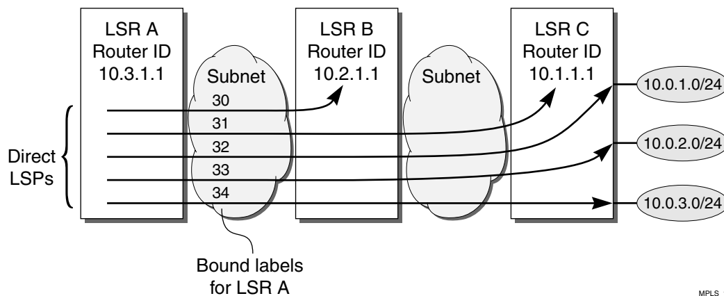
Figure 6-1: Direct and indirect LSPs
