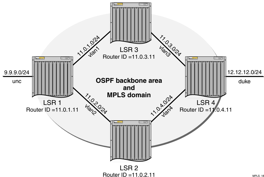
Figure 4-1: MPLS configuration example
