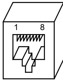
RJ-45 female
